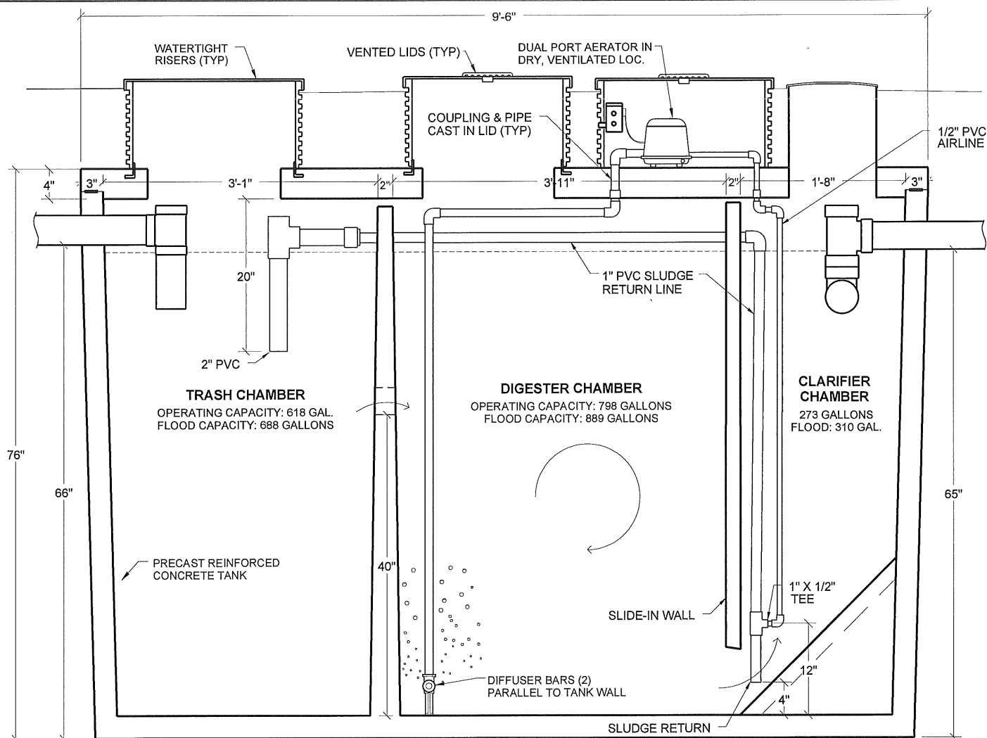
BNR-750 SIDE VIEW NO SCALE
