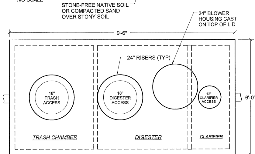
BNR-750 TOP VIEW NO SCALE
