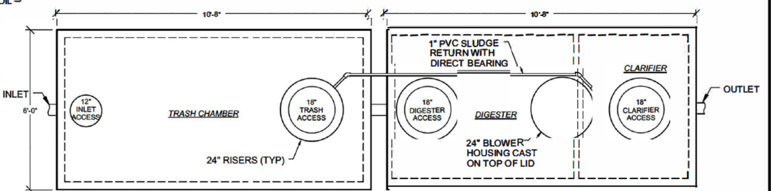
BNR-1500 TOP VIEW NO SCALE
