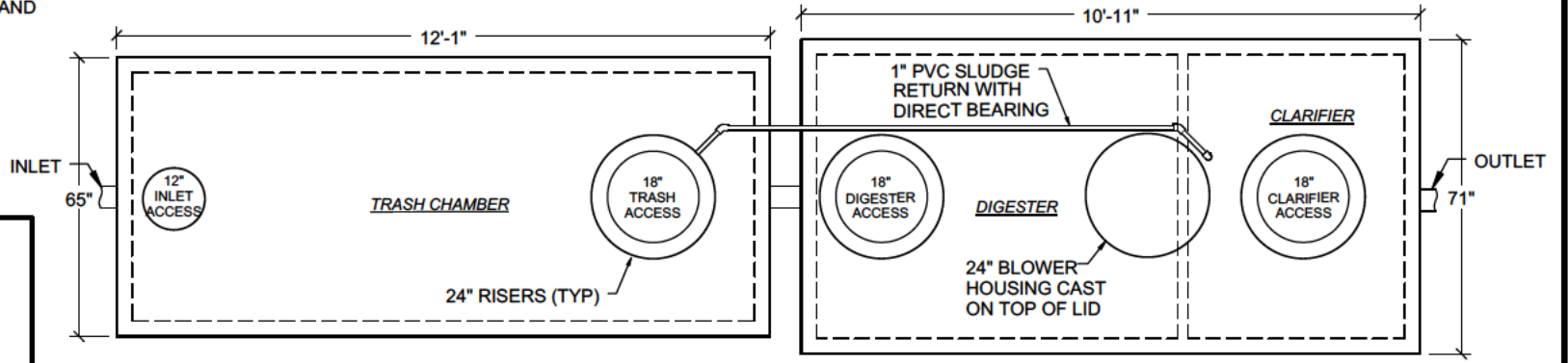
BNR-1500 TOP VIEW NO SCALE
