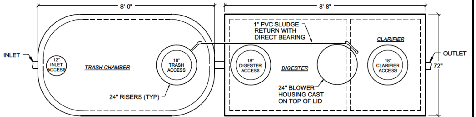
BNR-1000 TOP VIEW NO SCALE
