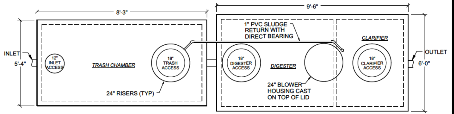
BNR-1000 TOP VIEW NO SCALE
