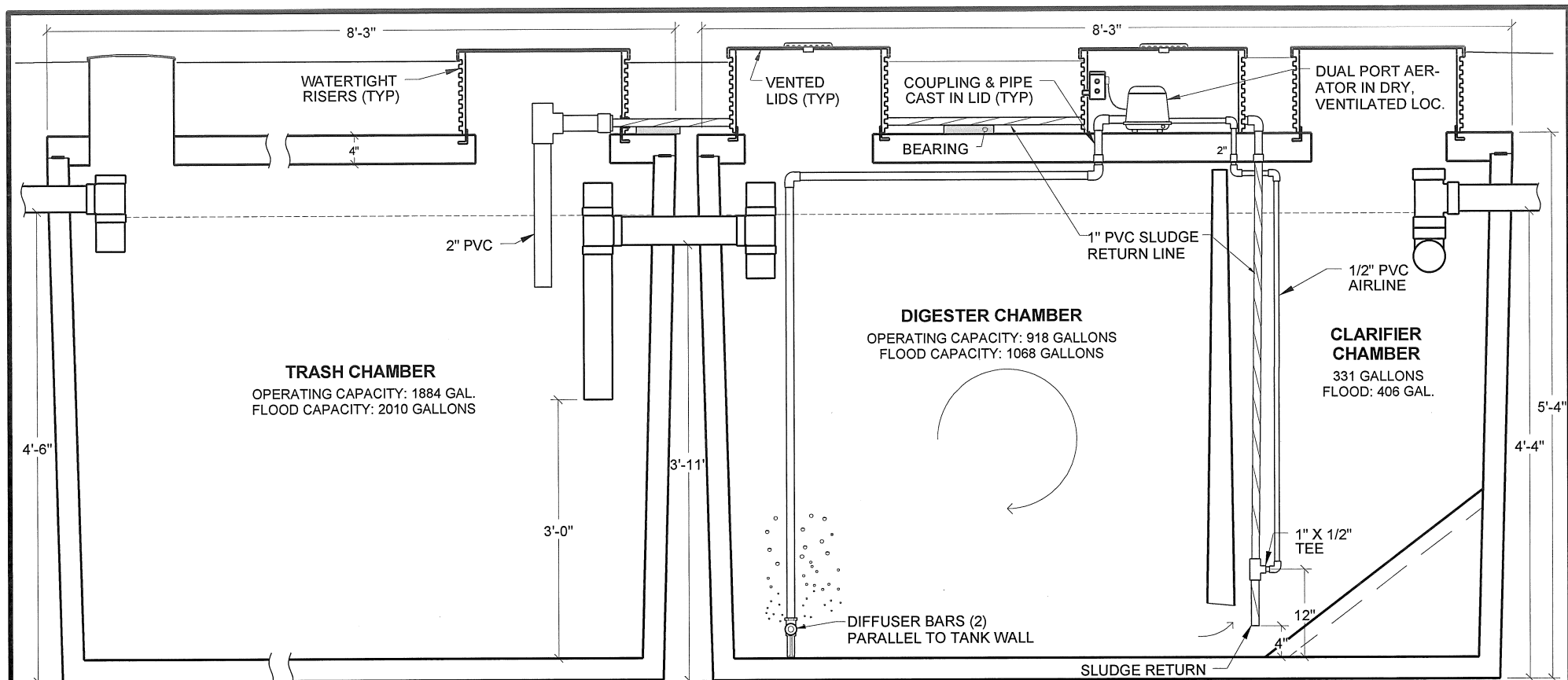
BNR-1000 SIDE VIEW NO SCALE
