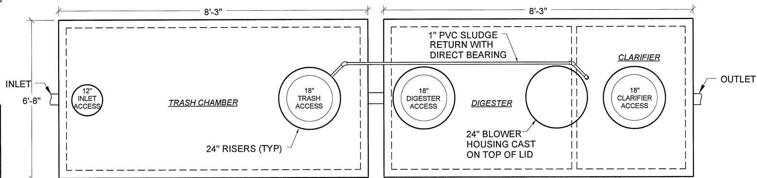
BNR-1000 TOP VIEW NO SCALE
