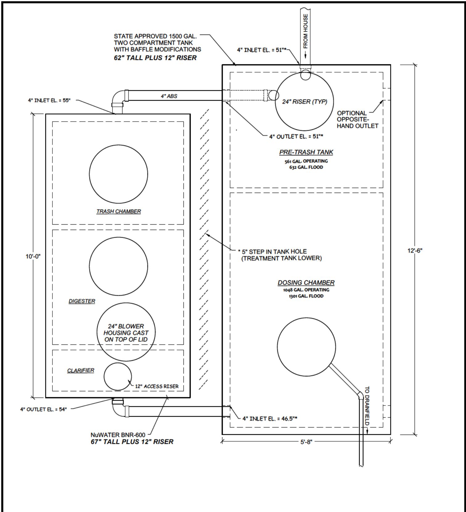
TOP VIEW SHOWING TANK CONFIGURATION WITH 1500 GALLON DOSE / TRASH TANK OPTION BERG VAULT VERSION
